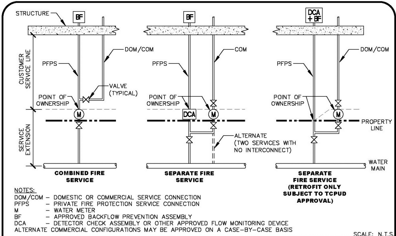
FIGURE 2 WATER ORDINANCE PRIVATE FIRE PROTECTION SERVICE CONFIGURATIONS
